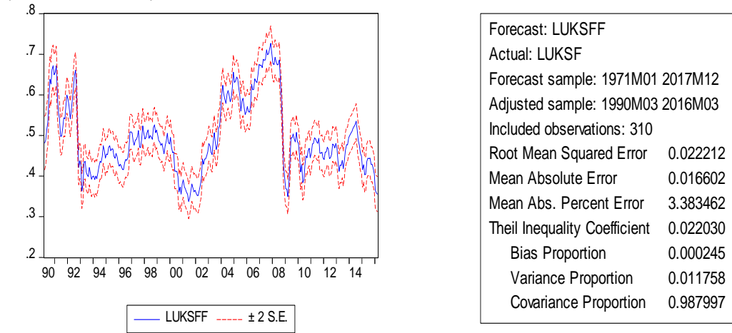
Figure 2b. Dynamic Forecast of the rp_{t+1}^e ($/£): Eq. (25), (24), and (27) (LUKSF-LUKF)
