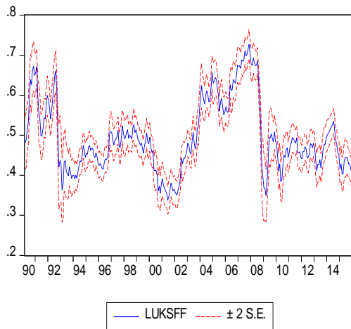
Figure 2a. Static Forecasting of the rp_{t+1}^e ($/£): Eqs (25), (24), and (27)
