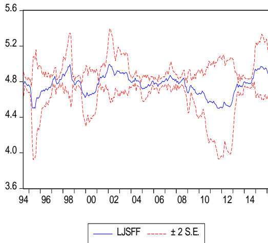
Figure 4a. Static Forecasting of the rp_{t+1}^e (¥/$): Eqs (25), (24), and (27)
