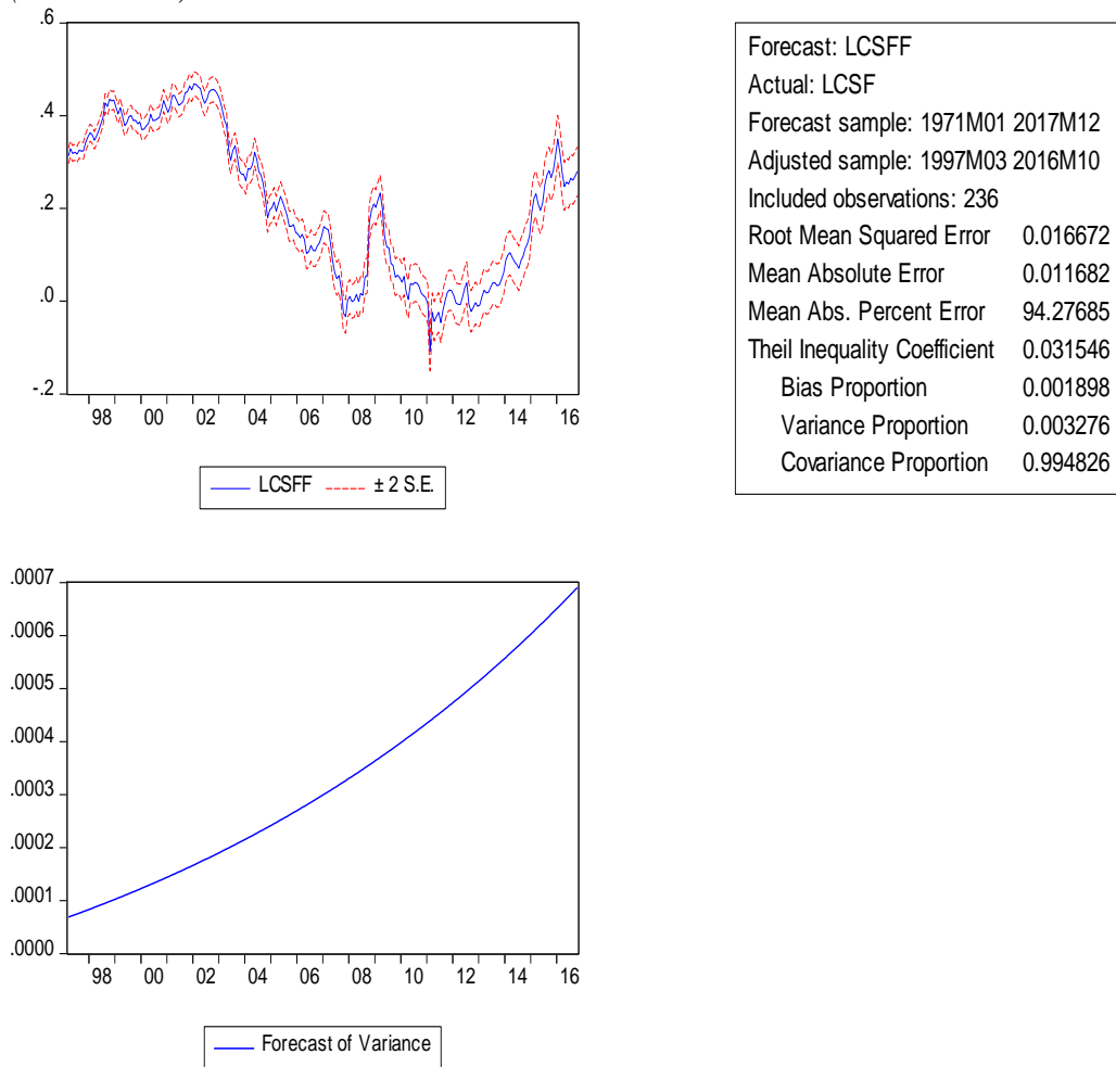
Figure 3b. Dynamic Forecast of the rp_{t+1}^e (C$/\$): Eq. (25), (24), and (27) (LCSF-LCF)
