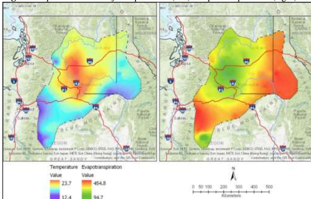
Figure 4. Spatial Patterns of Temperature (left) Evapotranspiration (right)
