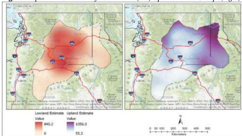
Figure 2. Spatial Distribution of Basin Floor (left) Upland Pollen Groups (right)
