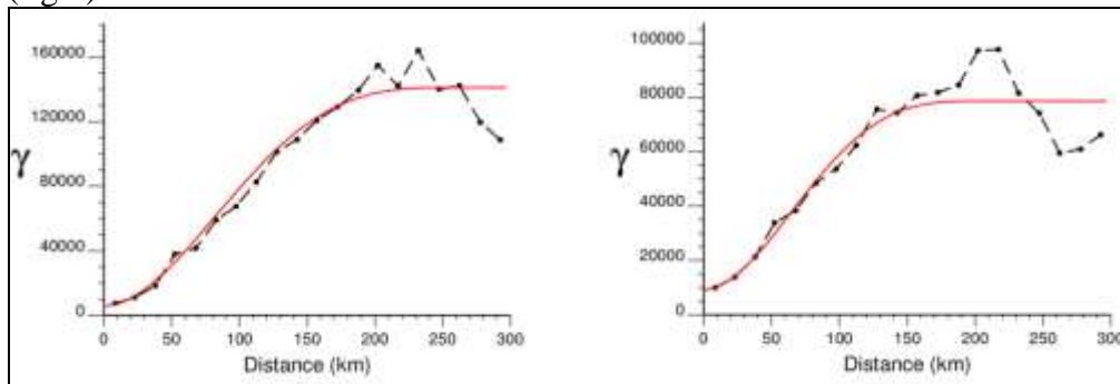
Figure 1. Cubic Variograms of the Basin Floor (left) Upland Pollen Groups (right)
