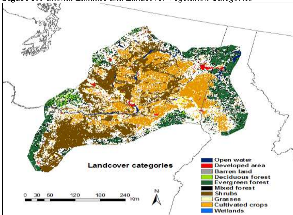
Figure 3. National Landuse and Landcover Vegetation Categories
