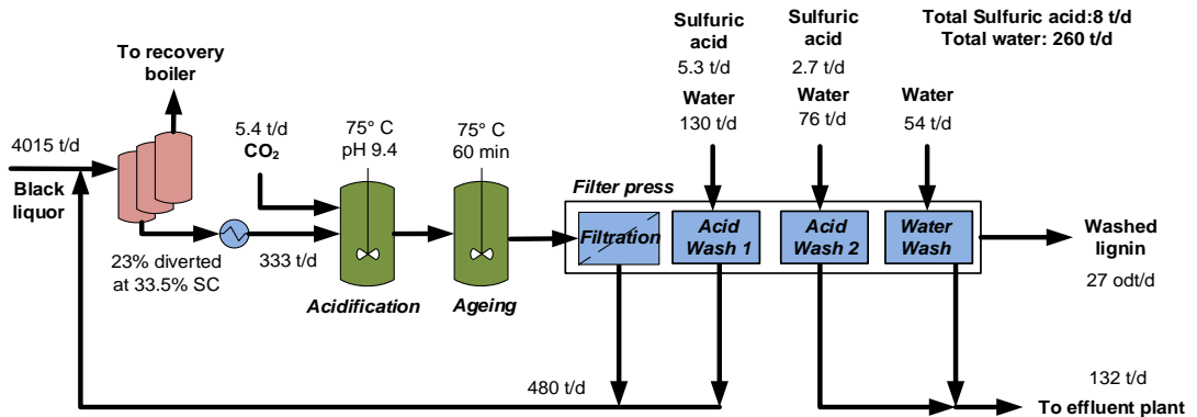
Figure 3. Process Flow Diagram for the Precipitation of Lignin by CO 2 Injection
