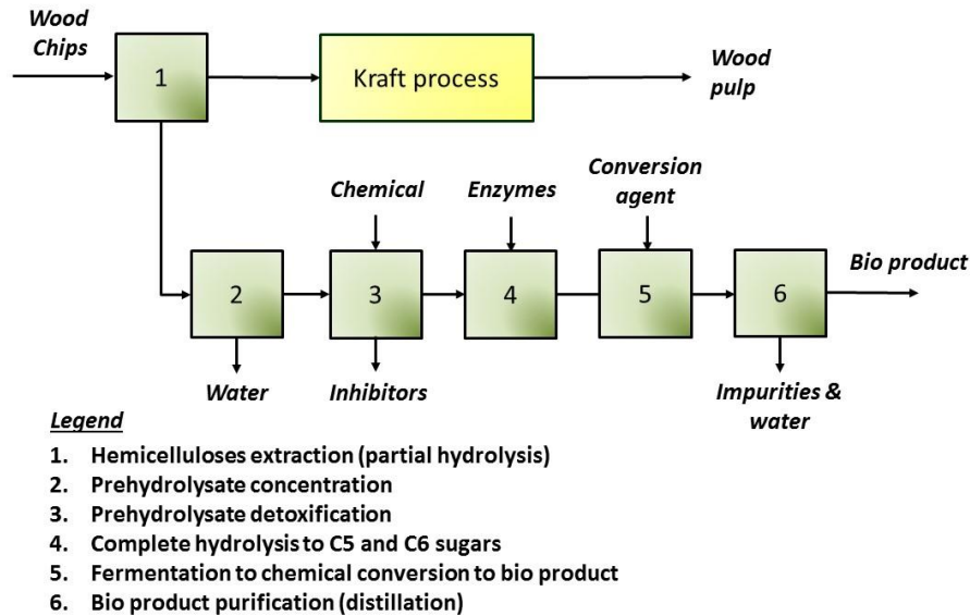
Figure 7. General Conversion Process of Hemicelluloses to Value Added Products
