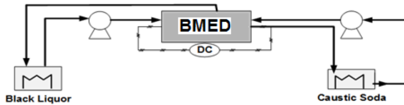
Figure 5. Schematic of a Black Liquor Acidification Process by Electro dialysis with Bipolar Membrane
