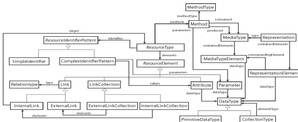
Figure 2. The Core of the Structural Metamodel
