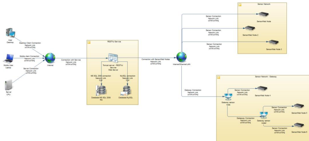
Figure 3. RESTful Sensor Web Infrastructure Diagram
