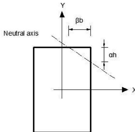
Figure 3. Column with the Neutral Axis Inclined to x-axis
