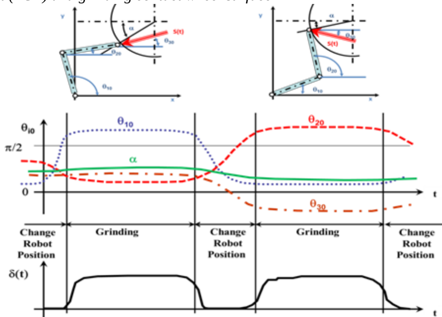
Figure 7. Typical robot parameters during grinding process. Path planning parameters result in the geometrical intersection \delta(t) of robot's tool center point (TCP) and grinding contact wheel surface
