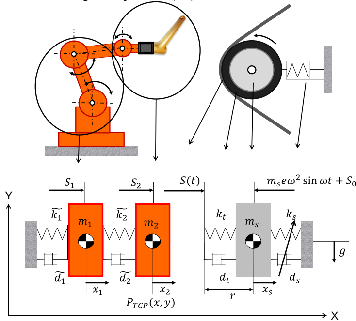
Figure 7. Lumped Parameter Model for numerical simulation. All DOFs are translational according to Equation (22)
