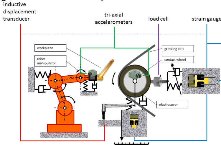
Figure 8. Measurement Setup
