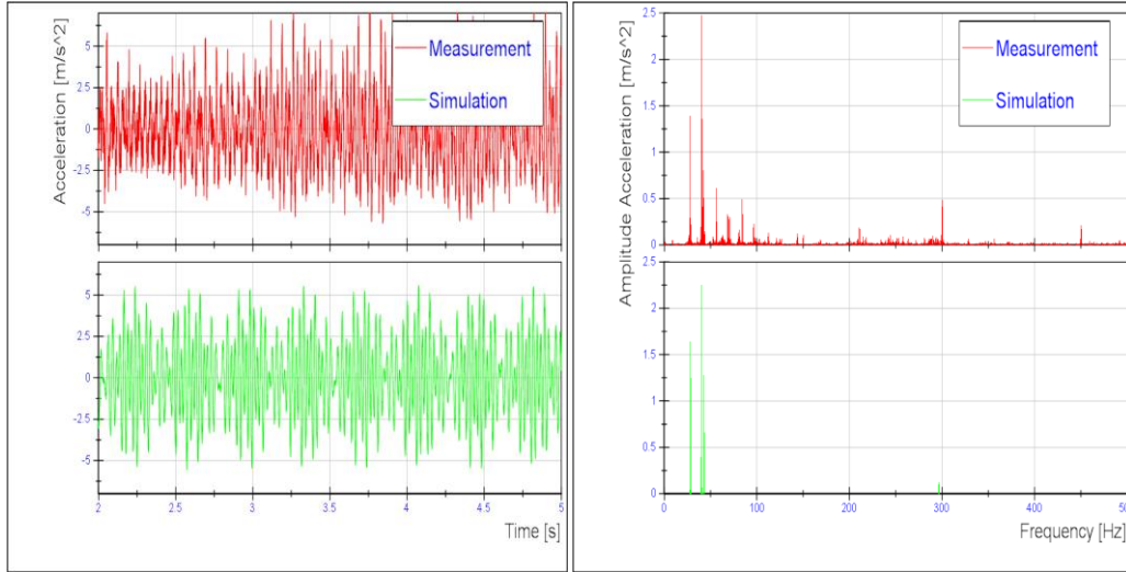
Figure 12. Comparing Measurement with Simulation in Time and Frequency Domains
