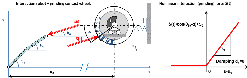
Figure 6. Nonlinear Interaction between the Robot and the Grinding Contact Wheel, Geometrically and Contact Force Driven
