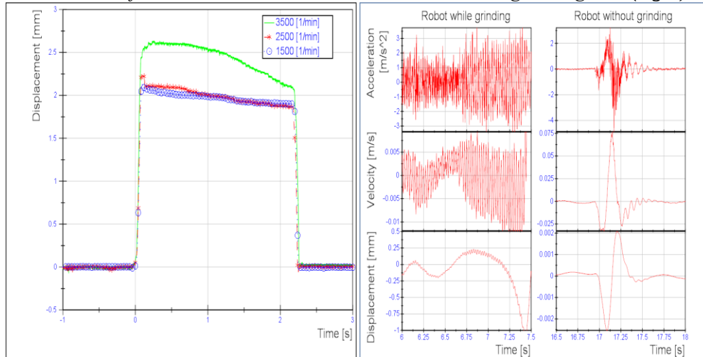
Figure 10. Displacement measurement x_s compared for different frequencies f while moving along the same path (left). Measurements of the robot comparing the behavior of the robot's TCP while in contact with the grinding belt (right)
