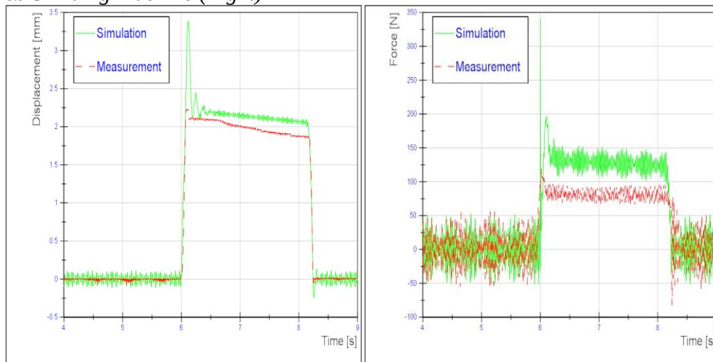
Figure 9. Displacement of the Contact Wheel (Left). Acting Force, Measured at Grinding Machine (Right)
