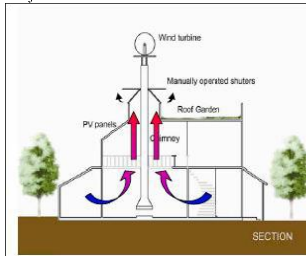
Figure 3. Section of the House
