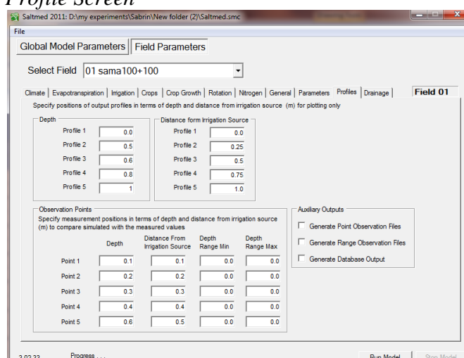
Photo 1. Soil Profile Screen
