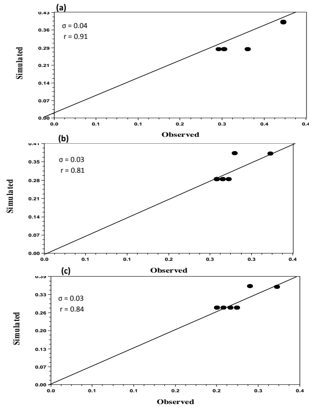
Figure 3. Comparison between Simulated and Observed Salinity Concentration in the Soil Profile of 75% Etc Water Regime with (a) 100% of the N Fertilizer, (b) 75% of the N Fertilizer, and (c) 50% of the N Fertilizer Treatments
