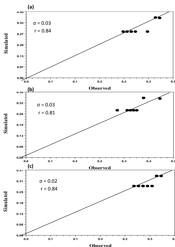
Figure 4. Comparison between Simulated and Observed Salinity Concentration in the Soil Profile of 50% Etc Water Regime with (a) 100% of the N Fertilizer, (b) 75% of the N Fertilizer, and (c) 50% of the N Fertilizer Treatments
