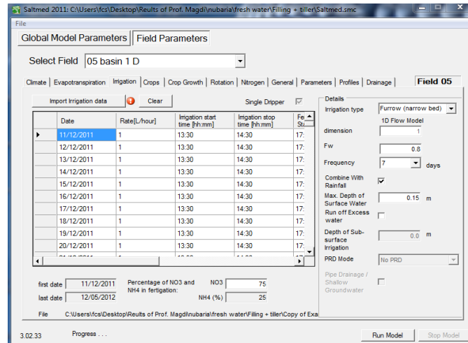
Photo 3. Irrigation Inputs Screen
