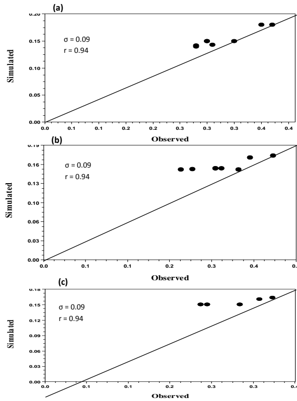
Figure 2. Comparison between Simulated and Observed Salinity Concentration in the Soil Profile of 100% Etc Water Regime with (a) 100% of the N Fertilizer, (b) 75% of the N Fertilizer, and (c) 50% of the N Fertilizer Treatments.
