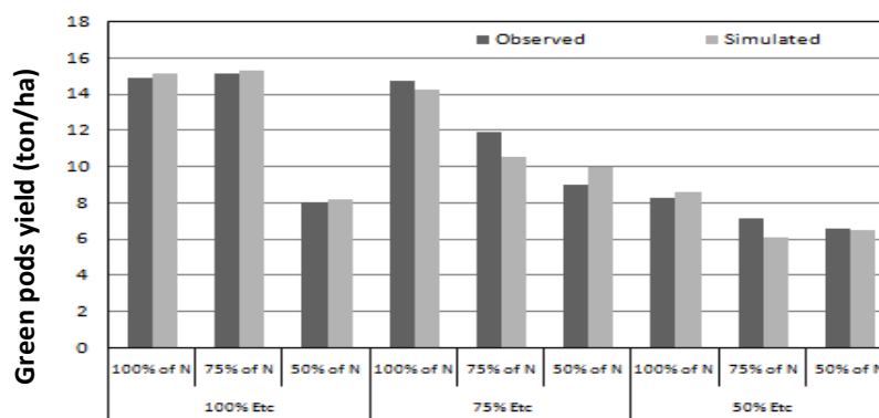
Figure 5. Simulated and Observed Green Pods Yield (ton/ha) under Different Experiment Conditions.
