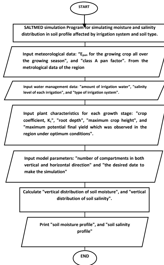
Flowchart 1. Flow Chart Components of SALTMED Simulation Model Program for Simulating Moisture and Salinity Distributions in Soil Profile Affected by Irrigation System and Soil Type
