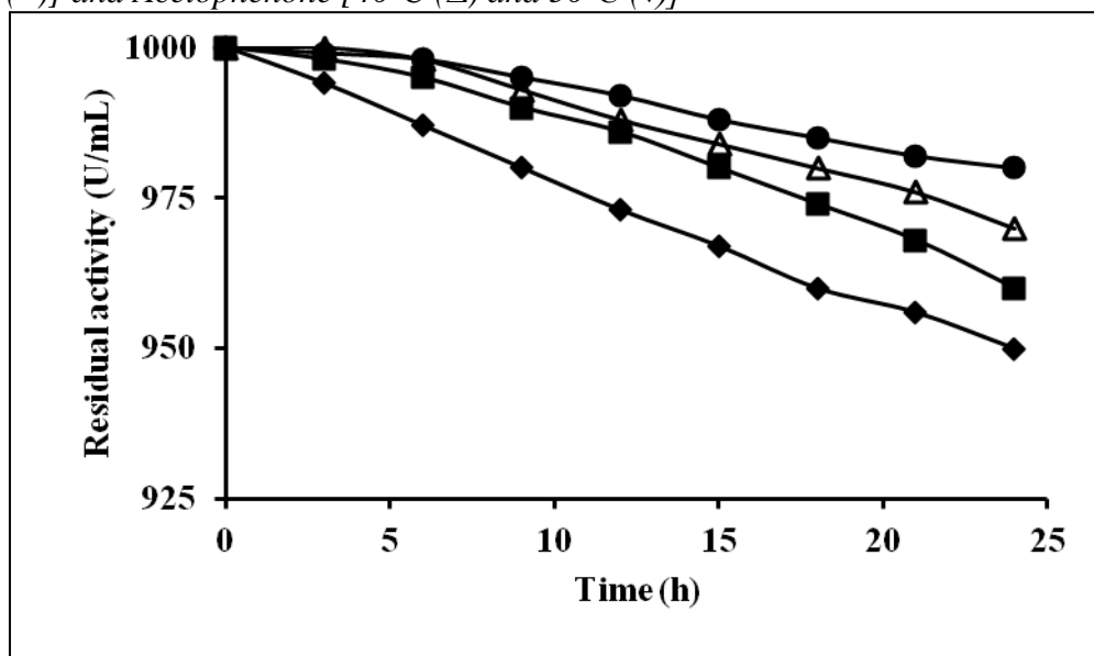
Figure 3. Variation of the Residual Activity of ADH Dissolved in 50mM Phosphate Buffer (pH 7.0), the Solution being maintained at 40°C and 50°C for 24h. The Enzyme Activity was Measured using 2-hexanone [40°C (●) and 50°C (■)] and Acetophenone [40°C (Δ) and 50°C (◆)]
