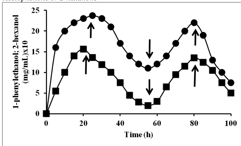
Figure 6. Profiles on the Continuous Conversion in the Membrane Reactor Fed with 10mM Acetophenone (●) and 10mM 2-hexanone (■), using Ethanol (10mM) as the Co-substrate. Conditions of Reaction: 30°C, Feeding Rate = 2mL/h, UF-membrane = 500Da, 100rpm and 50mM Phosphate Buffer [pH 7.0 (Ketone Solution) and pH 8.8 (Ethanol Solution)]. The Up-directed Arrows Indicate Ethanol Addition, whereas Down-directed Arrows Indicate Addition of Acetophenone or 2-hexanone
