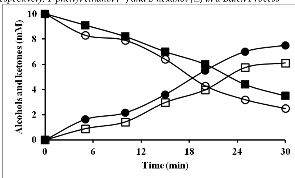
Figure 5. Conversion of Acetophenone (○) and 2-hexanone (■) into, Respectively, 1-phenyl ethanol (●) and 2-hexanol (□) in a Batch Process
