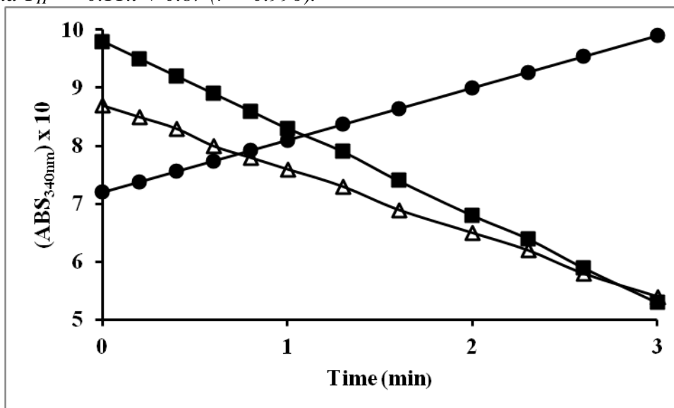
Figure 1. Alcohol Dehydrogenase Activity Measured by using Ethanol (●), Acetophenone (■) and 2-hexanone (Δ) as Substrates. The Least-square Linear Regression Equations for Ethanol, Acetophenone and 2-hexanone were, Respectively, Y_E = 9 \times 10^{-2}.t + 0.72 ( r = 0.997 ), Y_A = -0.15.t + 0.98 ( r = 0.994 ) and Y_H = -0.11.t + 0.87 ( r = 0.996 ).
