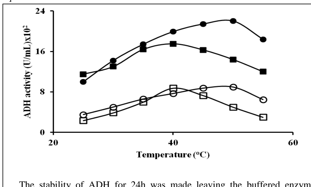
Figure 2. Variation of Alcohol Dehydrogenase Activity against the Temperature using Acetophenone [pH 7.0 (●) and pH 7.5 (○)] and 2-hexanone [pH 7.0 (■) and 7.5 (□)] as the Substrates. The Overall Reaction Time was Equal to 5min
