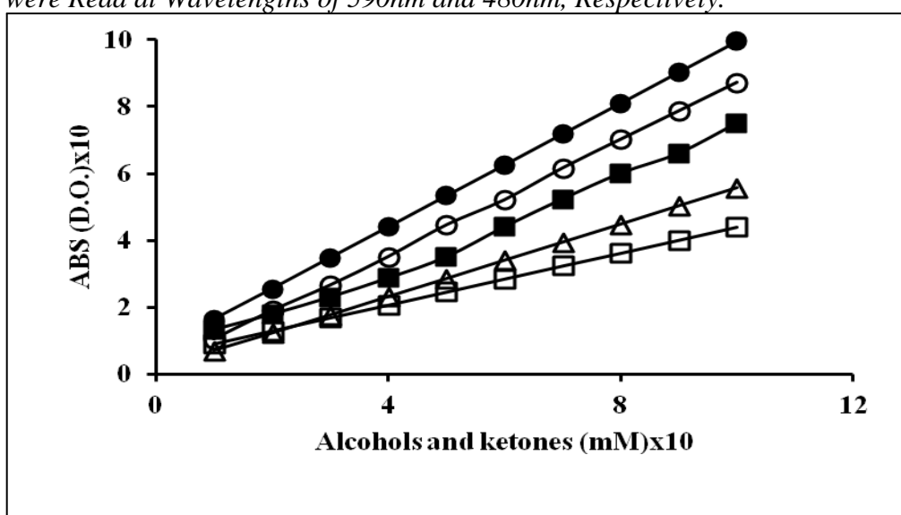
Figure 4. Standard Curves regarding the Determination of Alcohols [1-Phenylethanol (o), 2-hexanol ( \square ) and Ethanol ( \Delta )] and Ketones [Acetophenone ( \bullet ) and 2-hexanone ( \blacksquare )] by using, Respectively, Potassium Dichromate and 2,4-dinitro-phenylhydrazine Reagents, whose Color Intensities of Solutions were Read at Wavelengths of 590nm and 480nm, Respectively.
