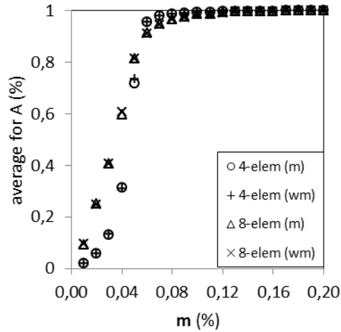
Figure 3. The change of the average concentration of A-agents, depending on the level of external field at the beginning of simulations, for p = 0,8 . The results are obtained for 4-elements and 8-elements neighbourhood and model with movement – (m), model without movement – (wm)
