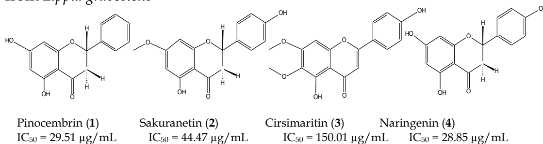
Figure 1. Structure and IC 50 against E. histolytica of flavonoids isolated from Lippia graveolens
